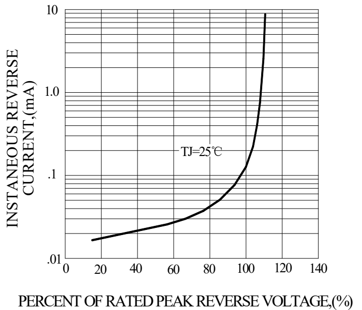
FIG.4-TYPICAL REVERSE CHARACTERISTICS
